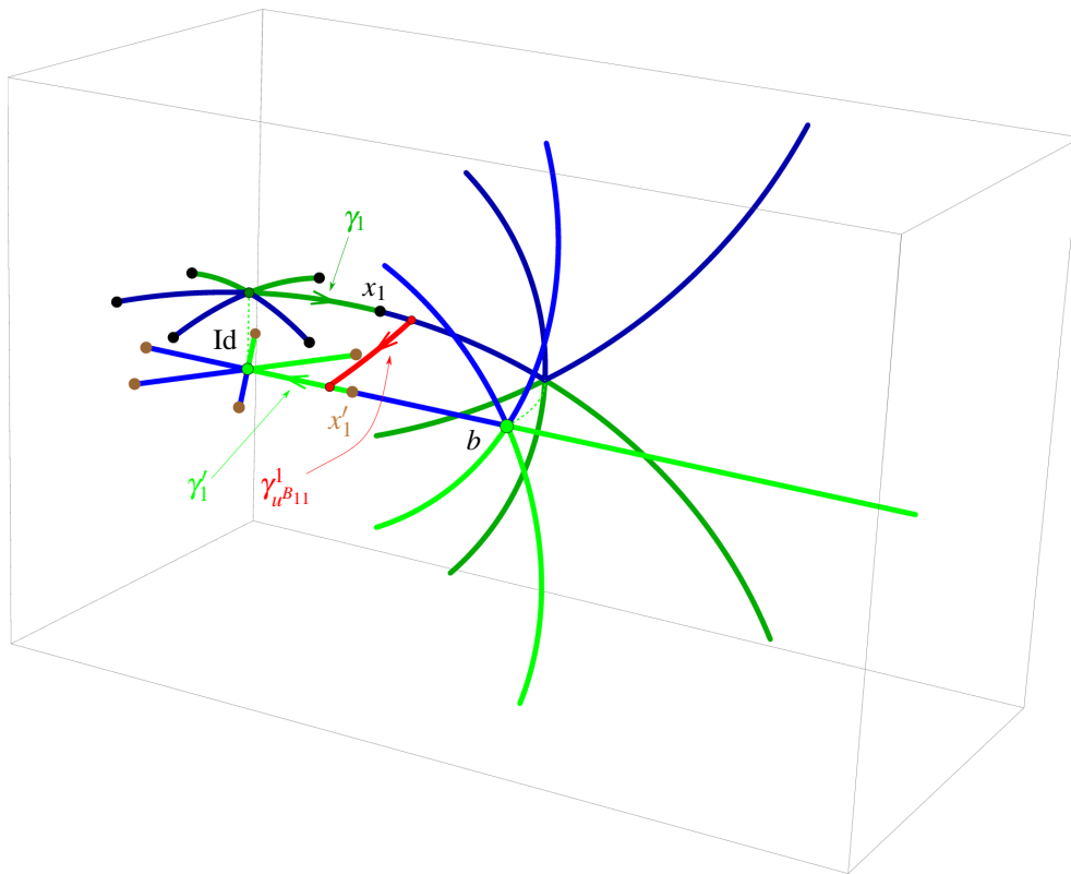
Figure 5.10: A lift of the path \gamma_{u^{B_{11}}}^1 with the fundamental domains centred at \text{Id} and b . From this plot one reads off that P_{\gamma_{u^{B_{11}}}^1} = \text{Id} .
