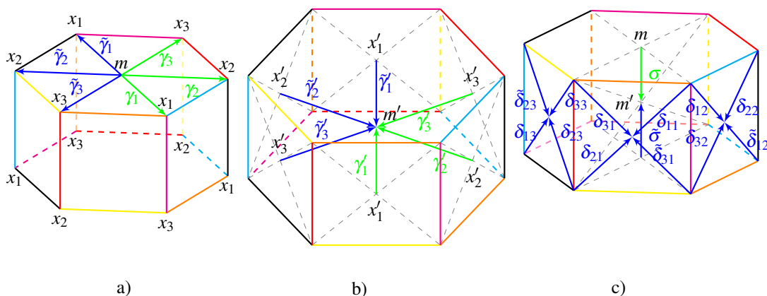
Figure 5.2: A Morse function f: L_\Delta \rightarrow \mathbb{R} . All flowlines of index 1 are depicted with arrows pointing in the direction of downward gradient flow. Note that in diagram c) the flowlines \delta_{ij} and \tilde{\delta}_{ij} always go from x_i to x'_j . The index 3 flowlines \sigma and \tilde{\sigma} and the different colouring (green and blue) of the flowlines will be used below for the calculation of parallel transport maps.
